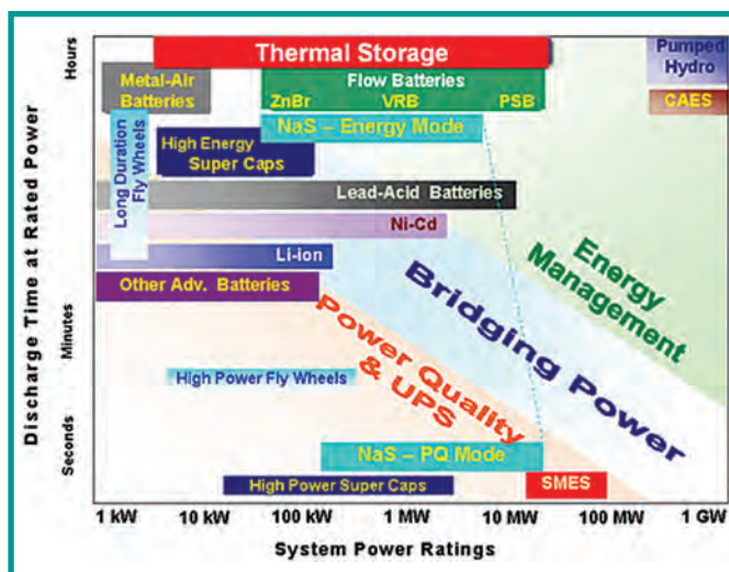
Figure 1: Different types of energy storage systems. 7
