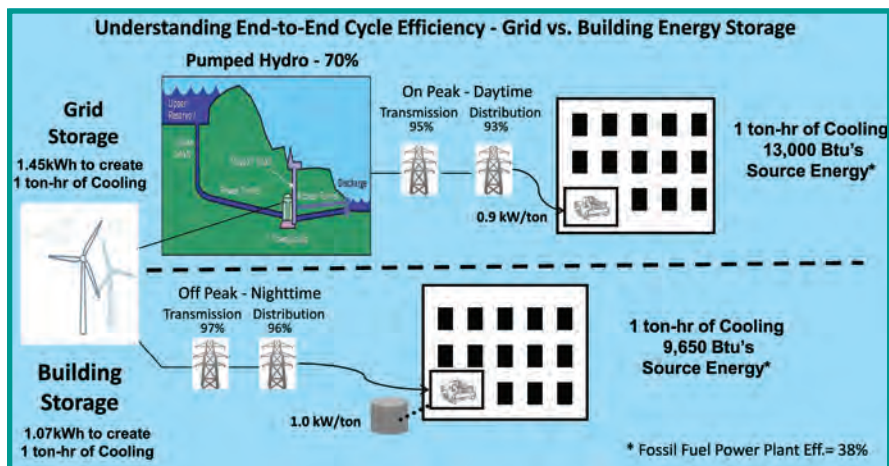
Figure 5: Energy storage and source energy for cooling.
