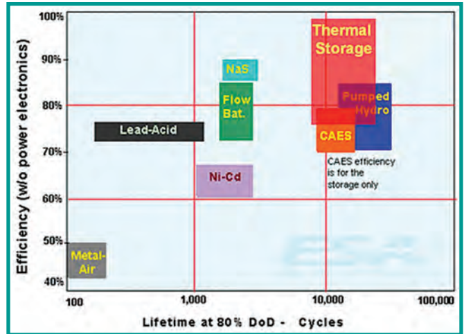
Figure 3: Cycle efficiencies and usable life expectance. 7
