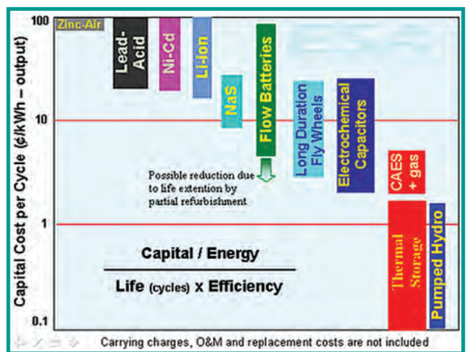
Figure 4: Total life costs of energy storage technologies. 7
