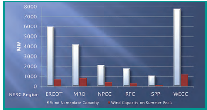
Figure 7: Storage bolsters variable wind resources. (Wind data from North American Electric Reliability Corporation, six of eight regions.)
