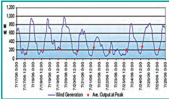
Figure 6: Design week wind generation output.
