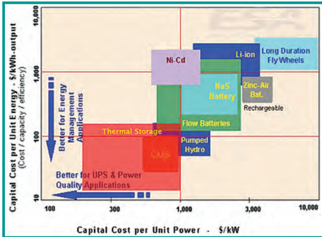
Figure 2: Energy storage system costs. 7
